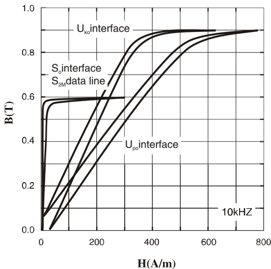
Typical B-H loop & inductance of S_{or} , S_{2M} , U_{KG} & U_{PO} interface pulse transformer
